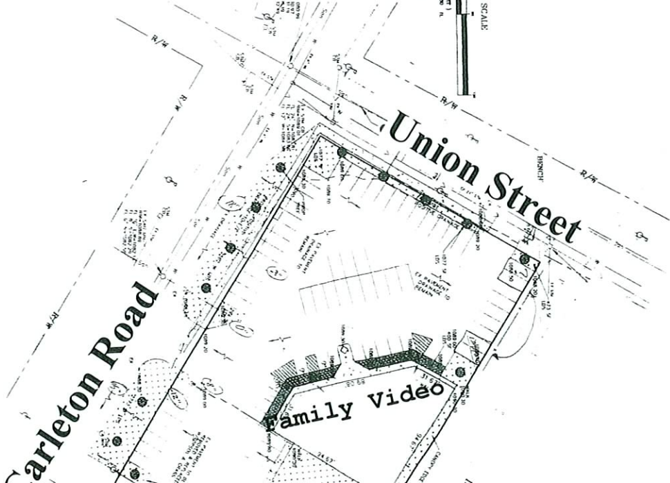
SITE GRADING PLAN
